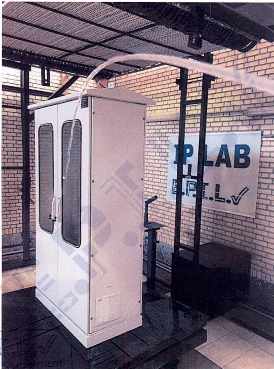
Figure 3: EUT under IPX5
